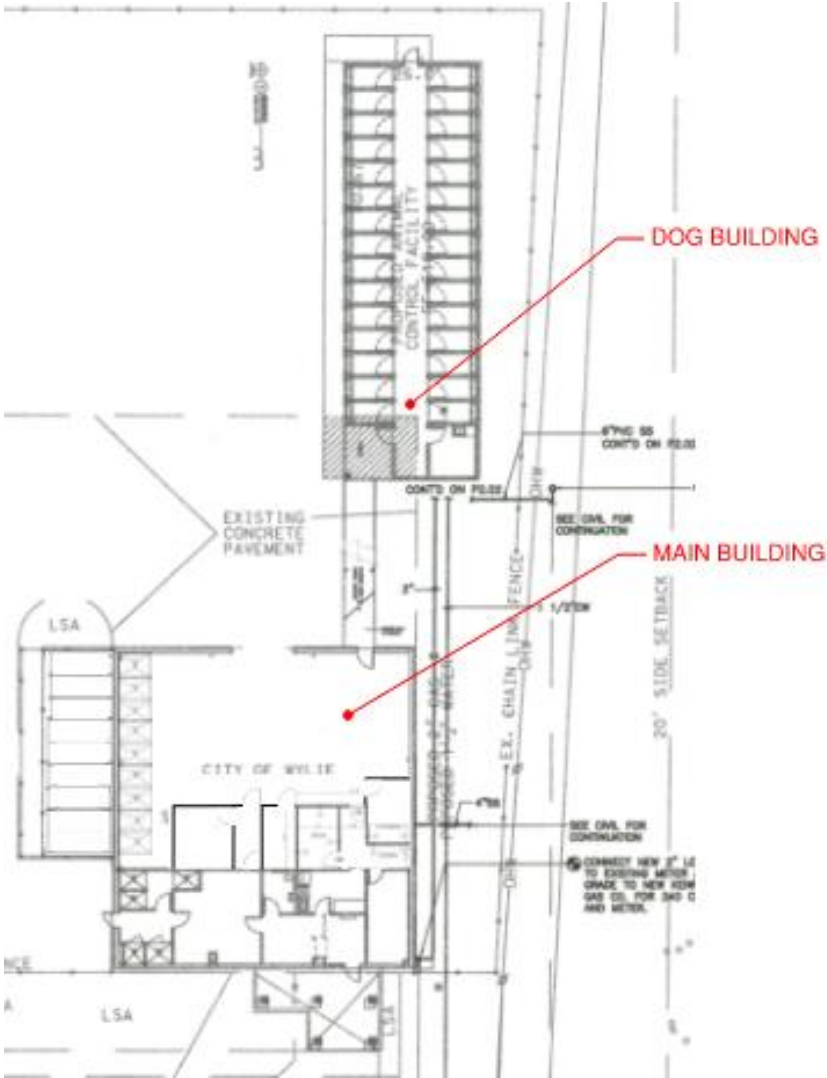
Layout of Existing Building
