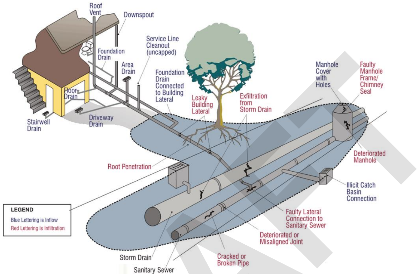
Figure 1 Typical Sources of I/I
