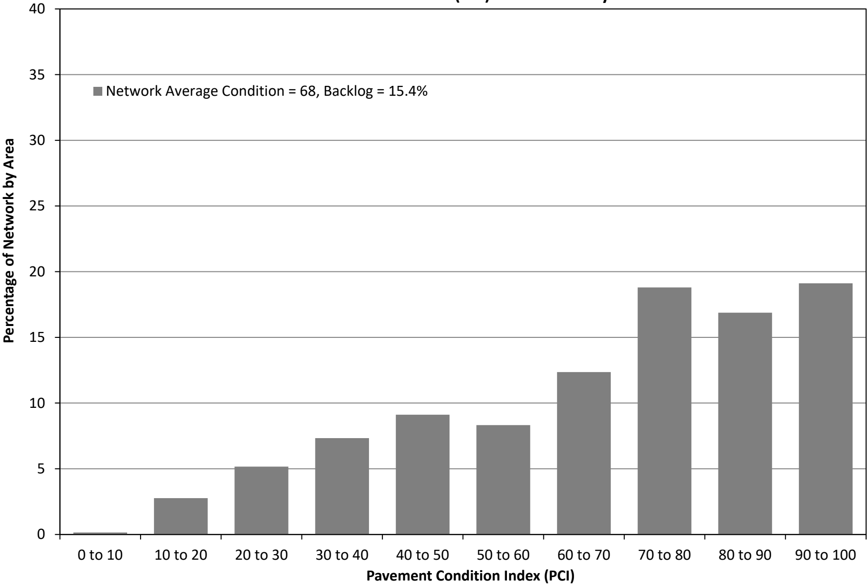
Pavement Condition Index (PCI) Distribution by Area
