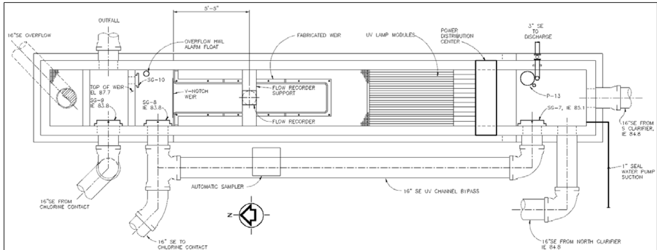
Figure 6-7. UV Disinfection
