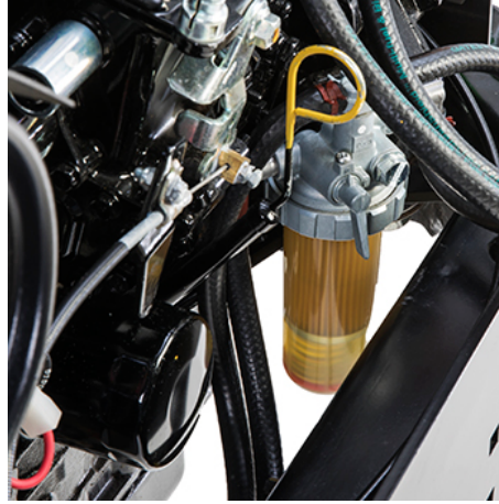
Engine oil filter, dipstick, and fuel filter/water separator
