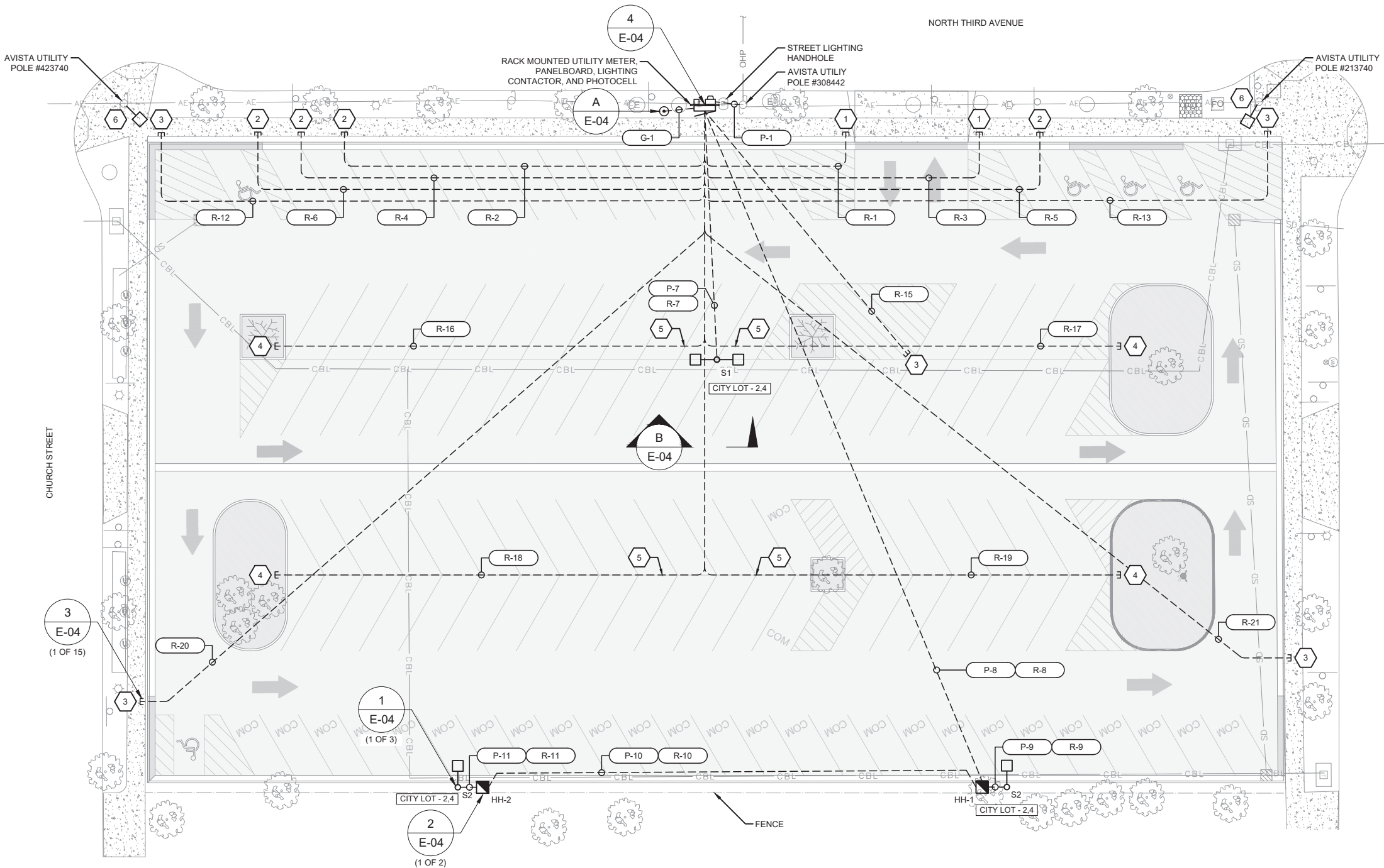
1 ELECTRICAL PLAN 1/16" = 1'-0" 0 8' 16' 32'
