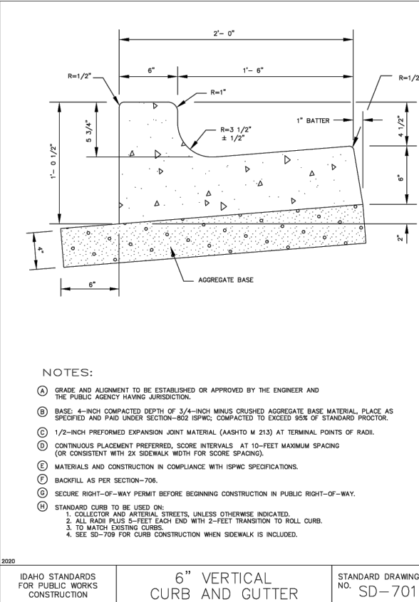
2 CURB AND GUTTER NOT TO SCALE
