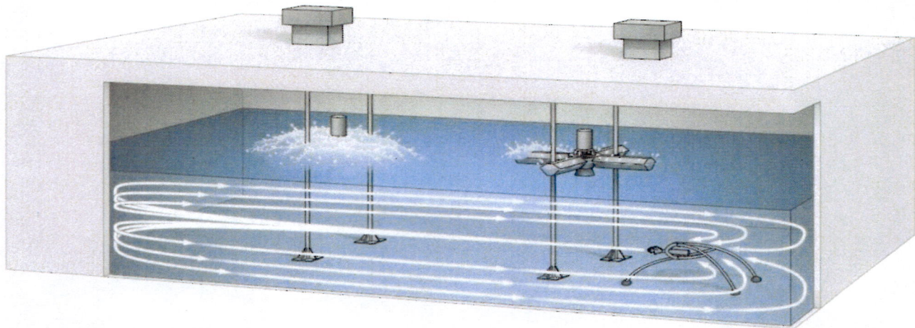
Customized aeration systems provide high rates of mass transfer to volatilize THMs out of any size or shape
