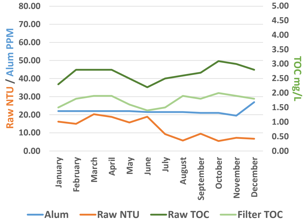
Alum PPM / Raw NTU / TOC Trend 2017
