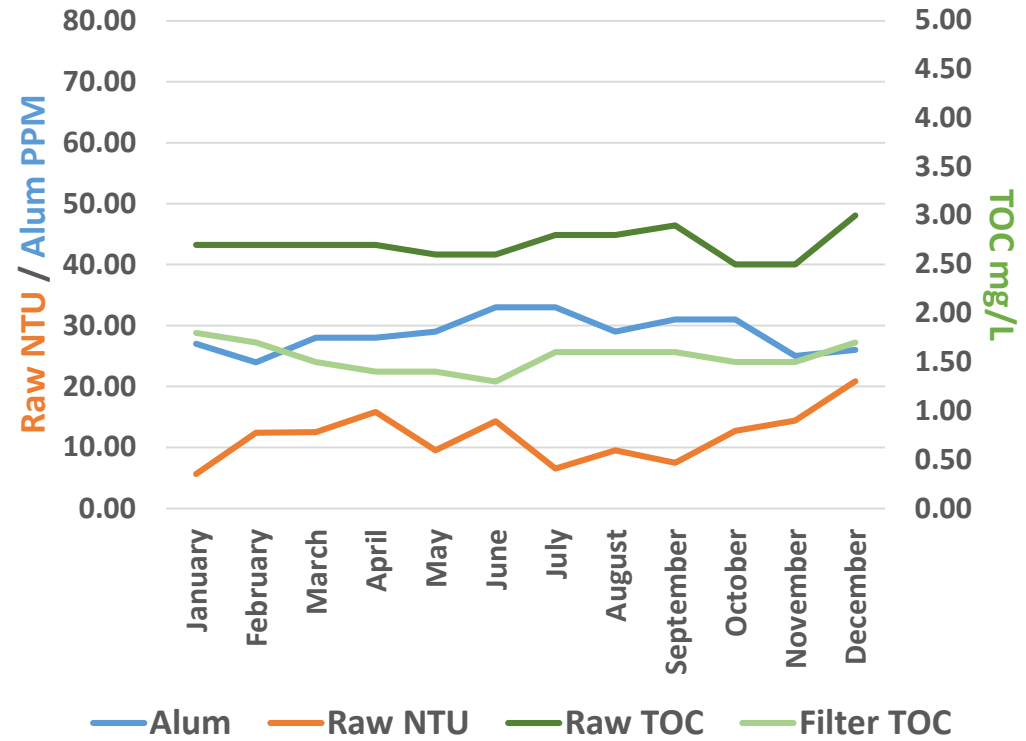
Alum PPM / Raw NTU / TOC Trend 2018
