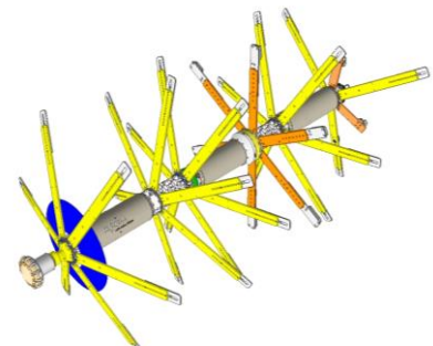
Figure 1: PipeDiver Inspection Platform for concrete pressure pipeline inspection
