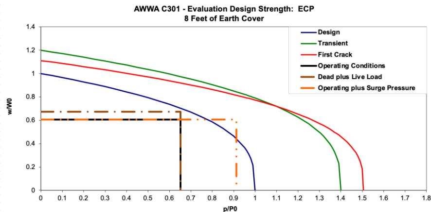
Figure 3: Structural Capacity
