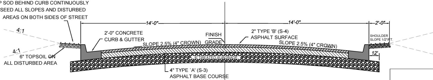
TYPICAL SECTION ASPHALT ROADWAY WITH CONCRETE CURB & GUTTER
