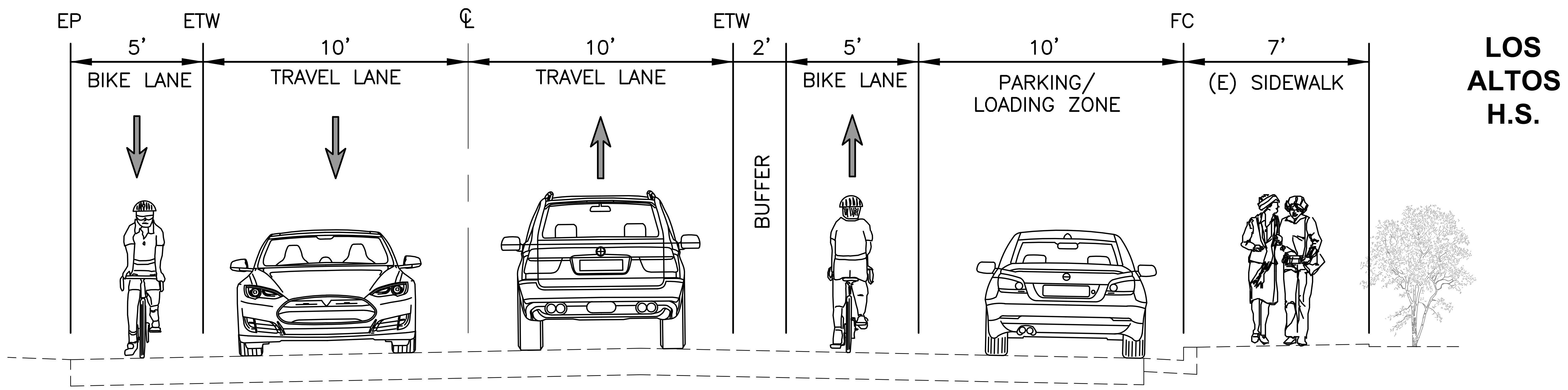
CONCEPT 4 JARDIN DRIVE PROPOSED CROSS SECTION - FACING EAST (VALENCIA DRIVE TO ALICIA WAY)
