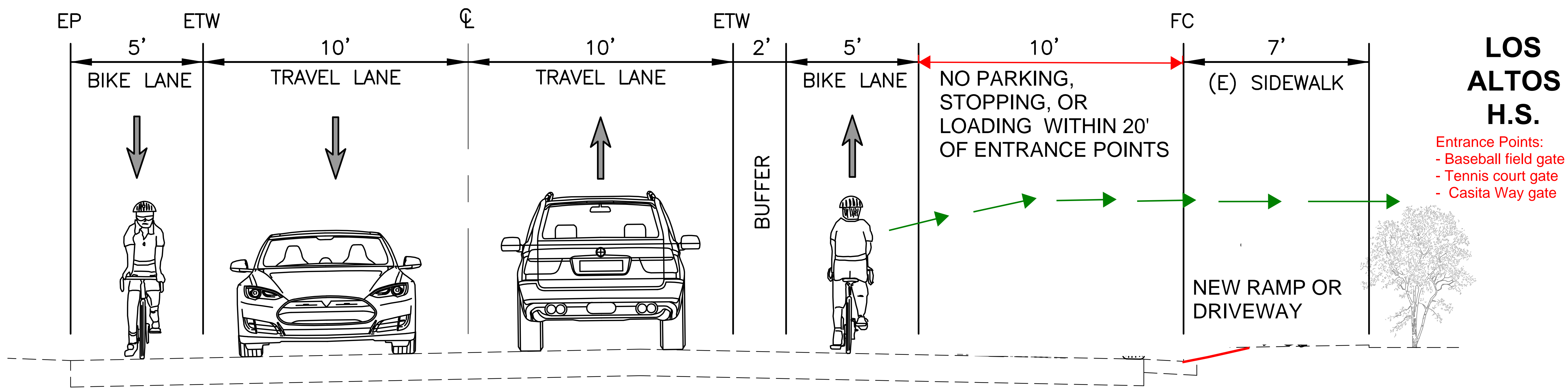
CONCEPT 4 JARDIN DRIVE PROPOSED CROSS SECTION - FACING EAST
