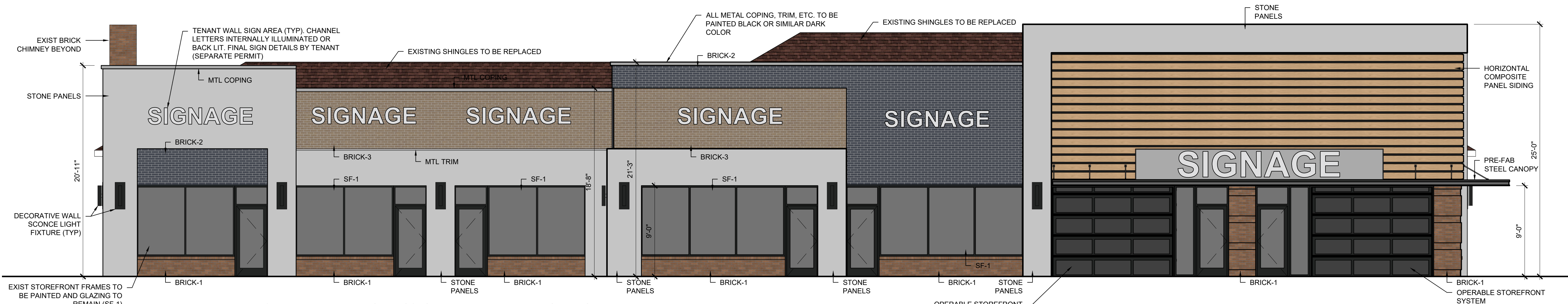
EAST ELEVATION (SOUTHFIELD ROAD) SCALE: 3/16" = 1'-0"
