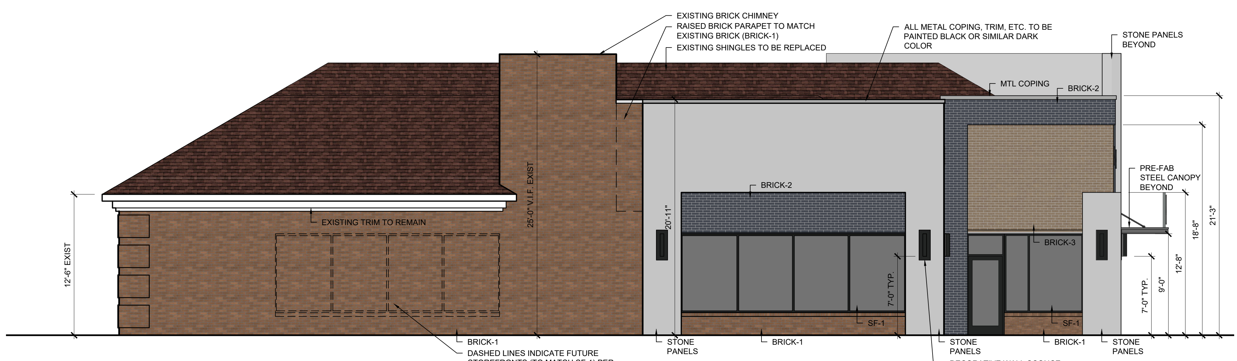
SOUTH ELEVATION (GOLDENGATE DRIVE) SCALE: 3/16" = 1'-0"
