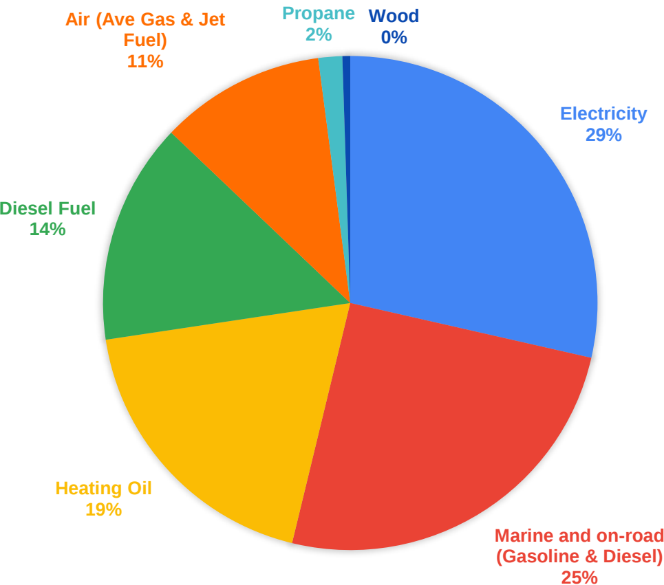
2021 COMMUNITY-WIDE ENERGY CONSUMPTION (SOURCE)
