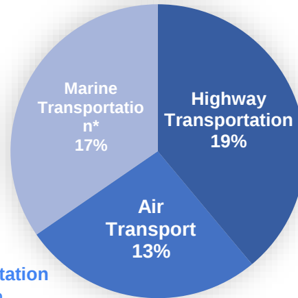
Transportation emissions breakdown
