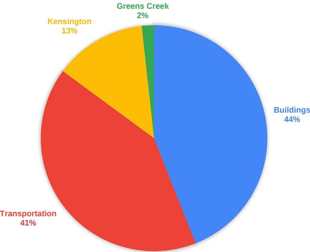
2021 COMMUNITY-WIDE ENERGY CONSUMPTION (SECTOR)
