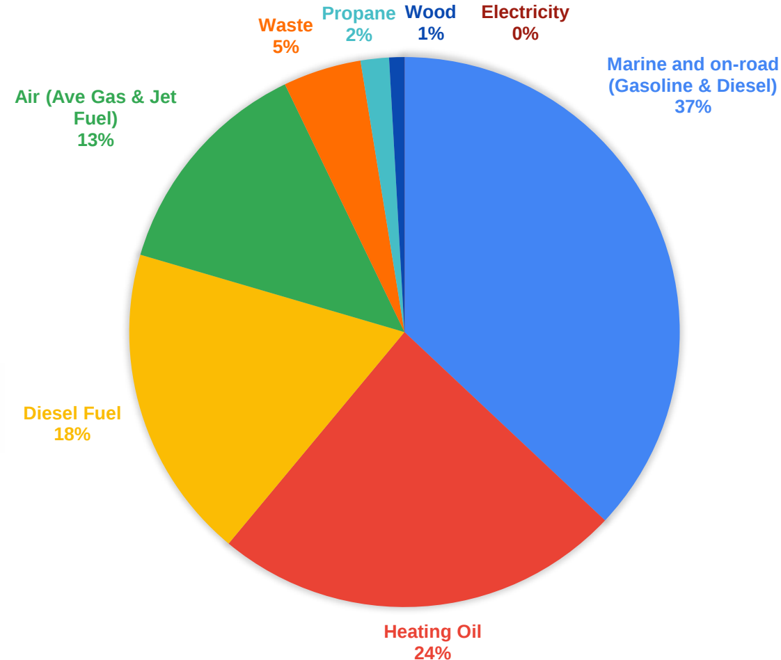
2021 COMMUNITY-WIDE GHG EMISSIONS (SOURCE)
