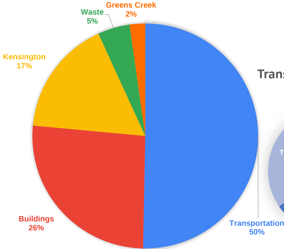
2021 COMMUNITY-WIDE GHG EMISSIONS (SECTOR)
