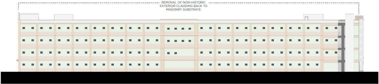
EXISTING WEST ELEVATION (POST DEMOLITION) NOT TO SCALE
