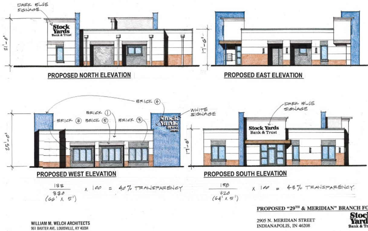
Proposed elevations for the bank
