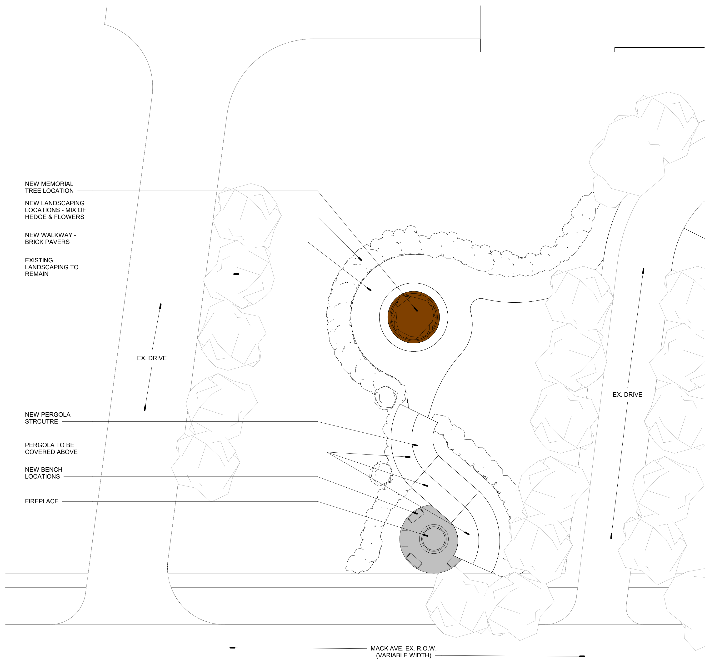
SITE PLAN - PERGOLA - FIREPLACE OPTION 1
