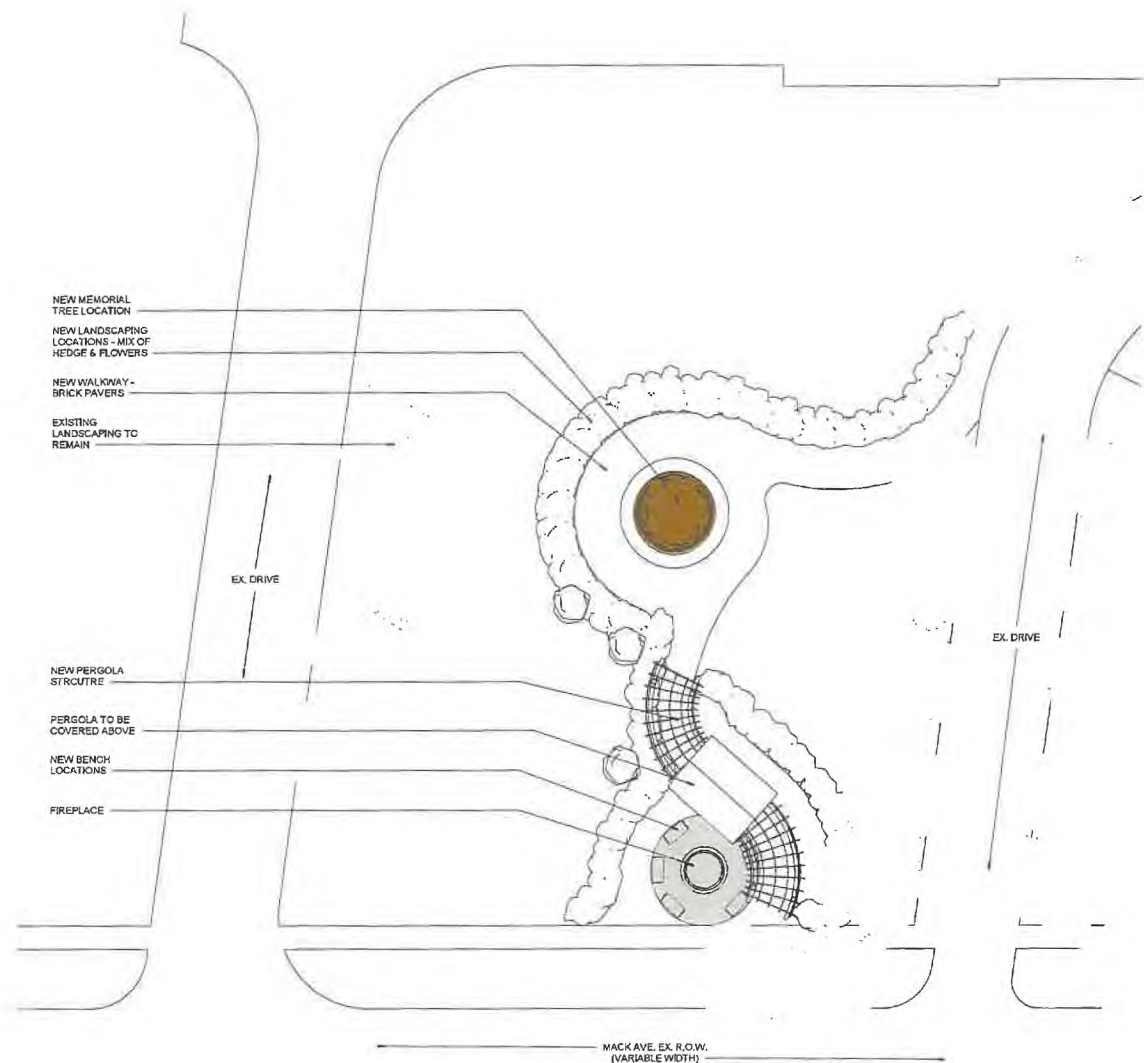
SITE PLAN - PERGOLA - FIREPLACE OPTION 1
