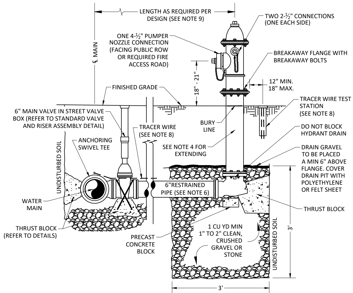
ELEVATION VIEW
