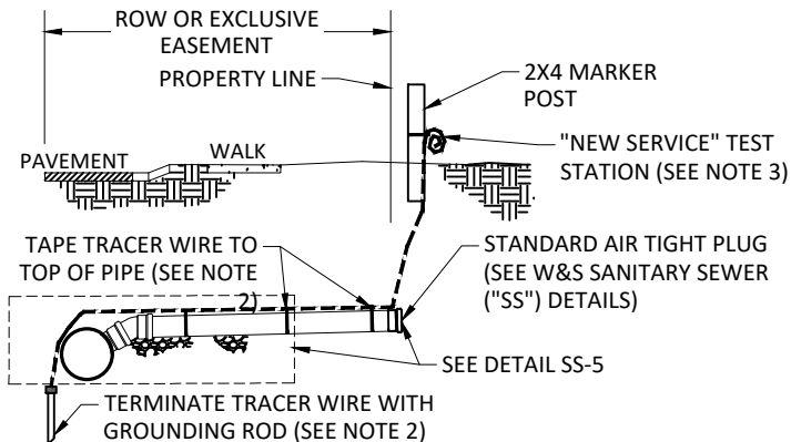
TRACER WIRE INSTALLATION - NEW CONSTRUCTION
