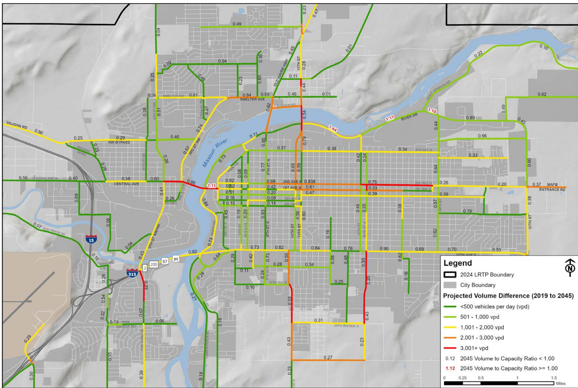
Figure 20: Projected Volume to Capacity Ratios
