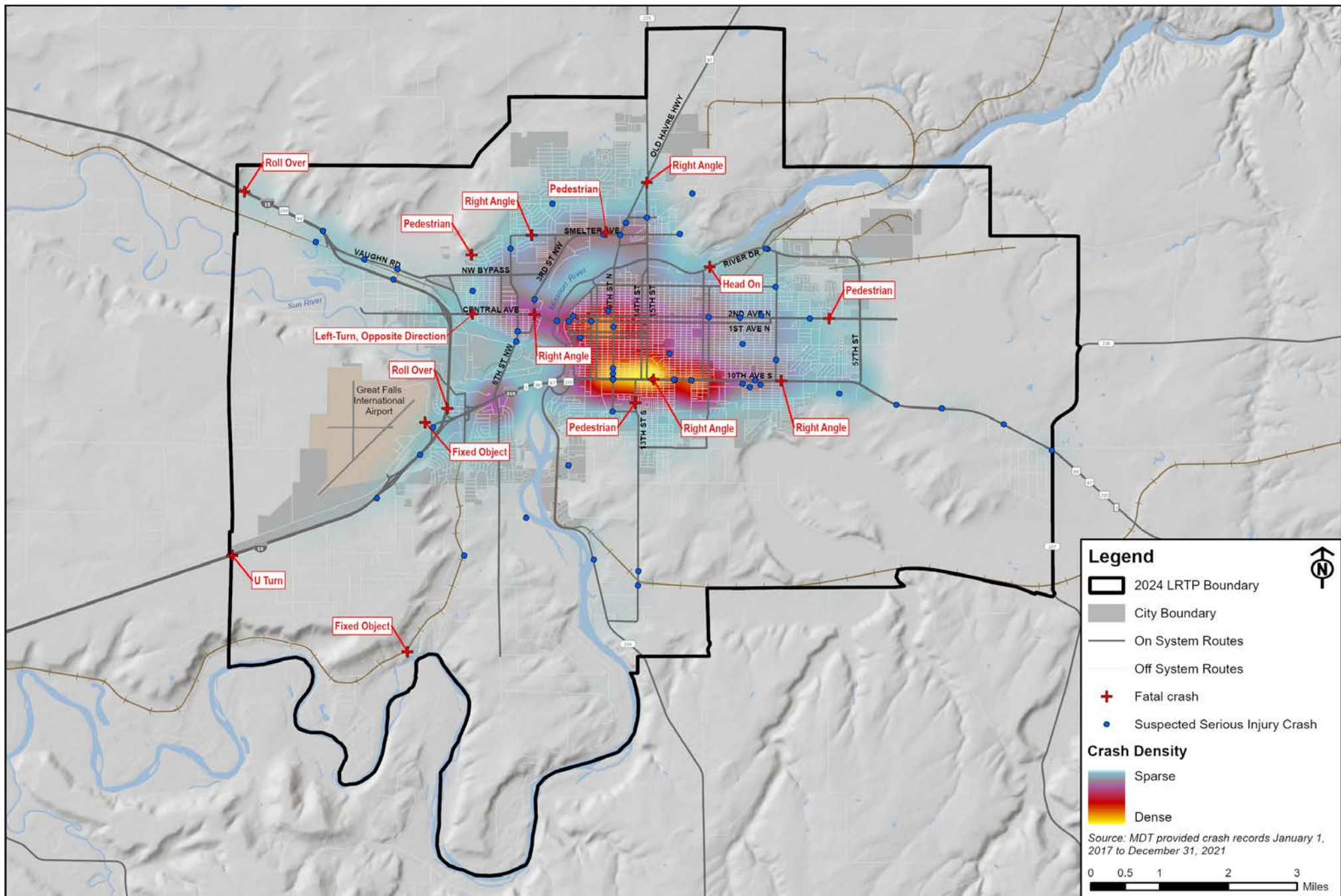
Figure 18: Crash Density
