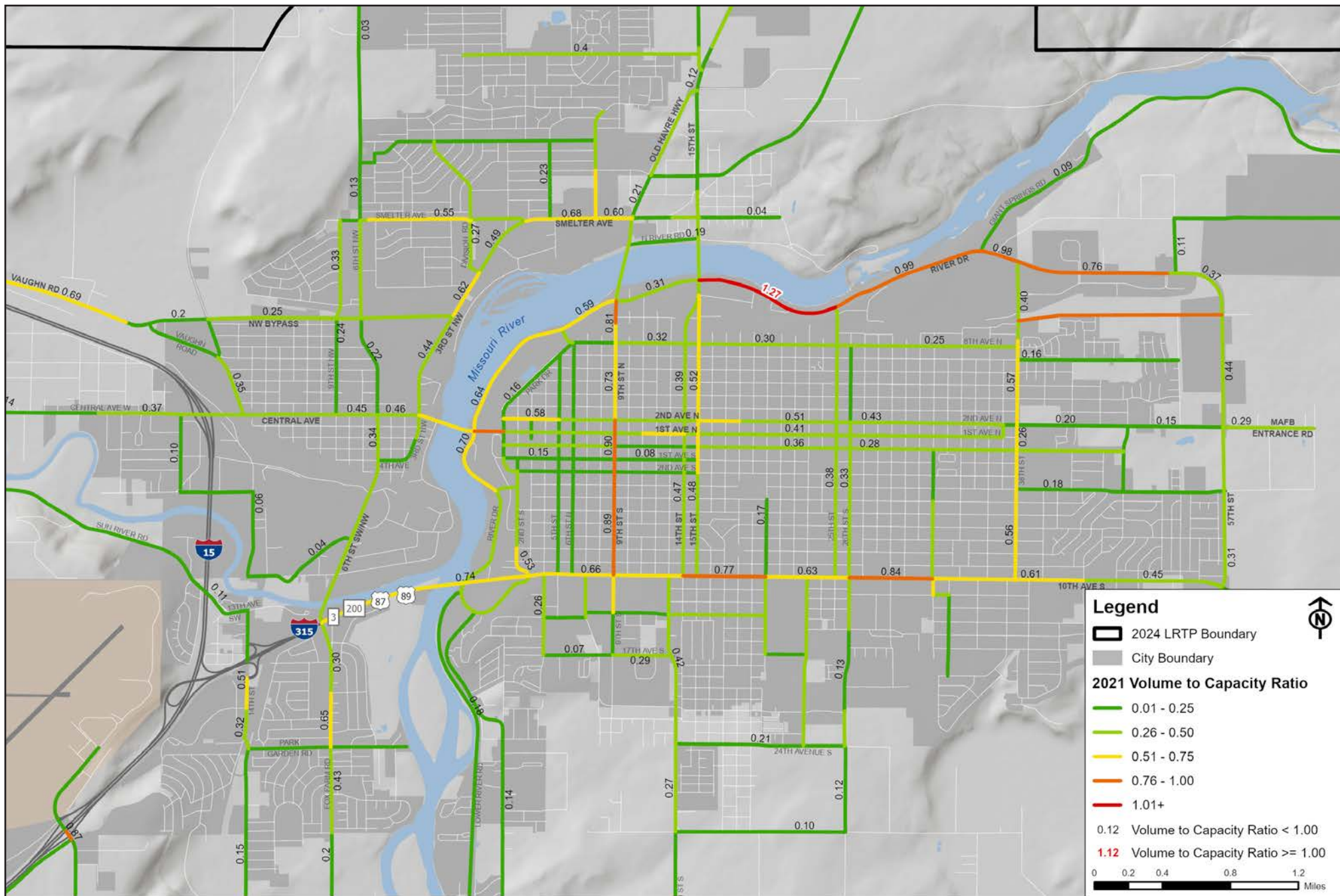
Figure 9: Existing Volume to Capacity Ratios
