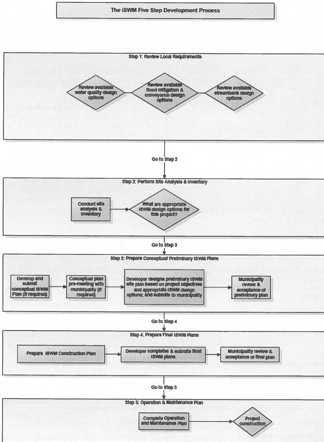
Figure 2.1 iSWM Flowchart
