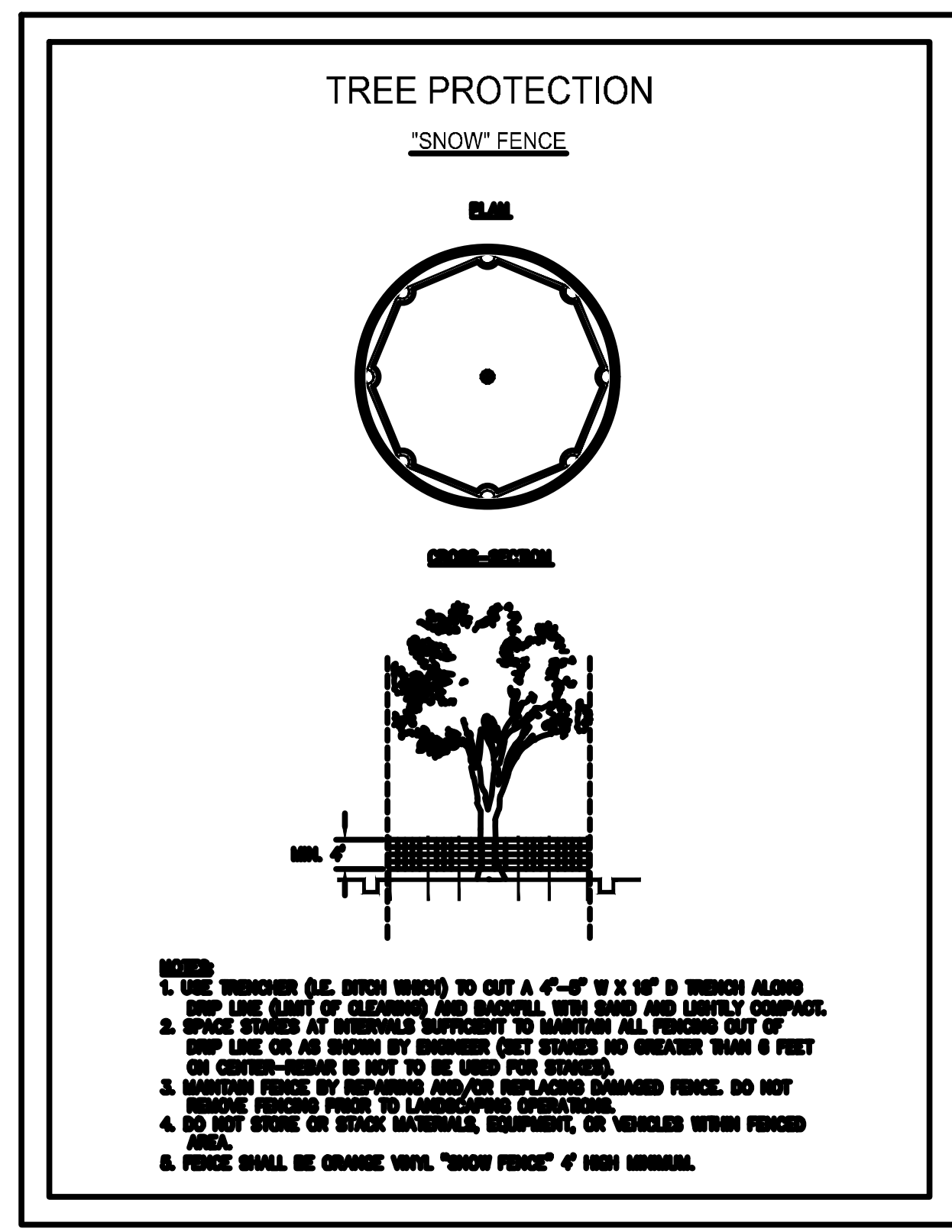
Tr TREE PROTECTION FENCE NTS
