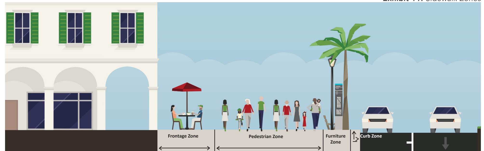
Exhibit 11. Sidewalk Zones
