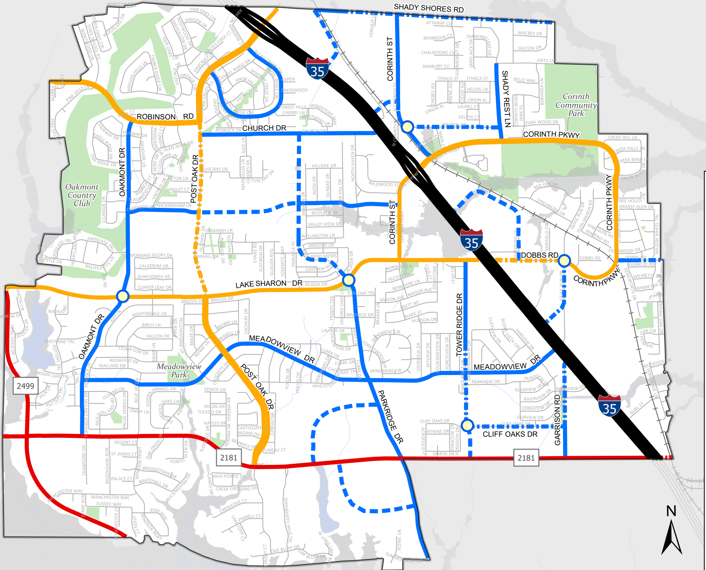
Exhibit 13. Corinth Master Thoroughfare Plan
