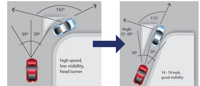
Sharper angles of slip lanes are important to slow cars and increase visibility. (Credit: Michele Weisbart)
