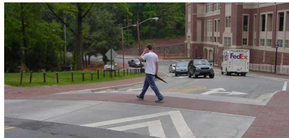
Raised crosswalk: University of North Carolina Campus, Chapel Hill, NC. (Credit: Ryan Snyder)
