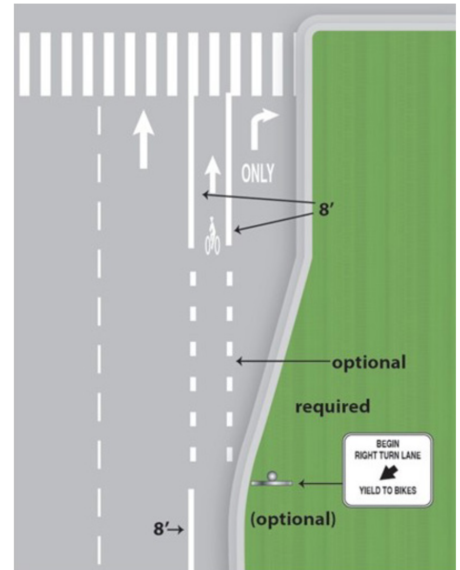
Bike lane markings at intersections with right-turn lanes. (Credit: Michele Weisbart)
