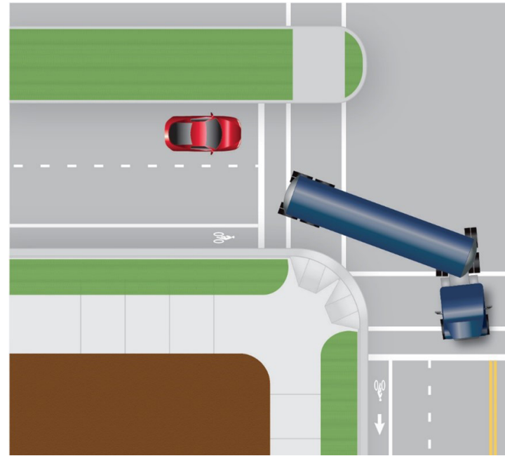
Corner radii can be kept smaller by allowing trucks and buses to turn into multiple receiving lanes. (Credit: Michele Weisbart)
