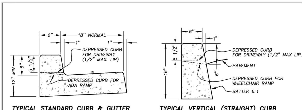
TYPICAL STANDARD CURB & GUTTER TYPICAL VERTICAL (STRAIGHT) CURB
