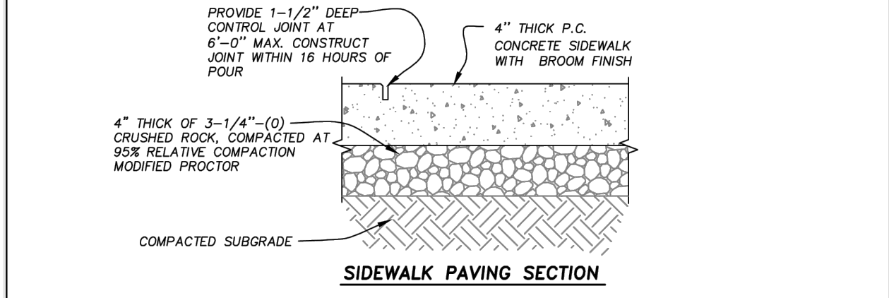
SIDEWALK PAVING SECTION
