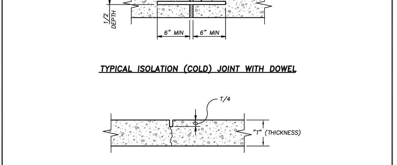
TYPICAL CONTRACTION JOINT
