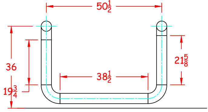
Section "C-C" Outlet Riser
