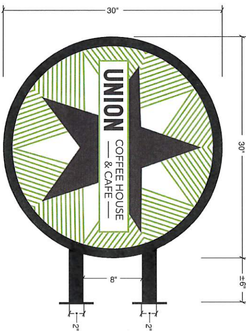
A LED ILLUMINATED DOUBLE FACED BLADE SIGN - OPTION 3 SCALE: 1 1/2" = 1'-0" SOFT: 6.25
