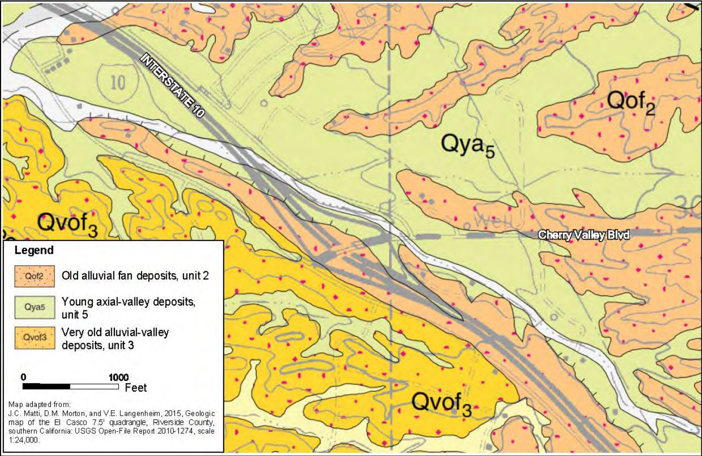
Figure 2.2.4-1: Geologic Units within the Project Vicinity
